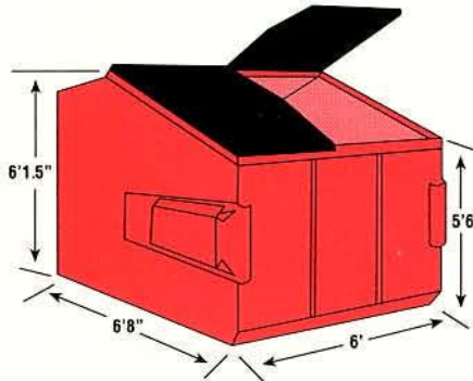
8 YARD CONTAINER
