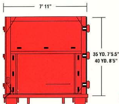
35 & 40 YARD COMPACTORS
