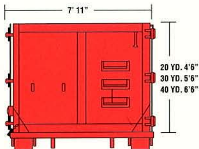
10, 20, 30, 40 YARD OPEN TOP CONTAINER
